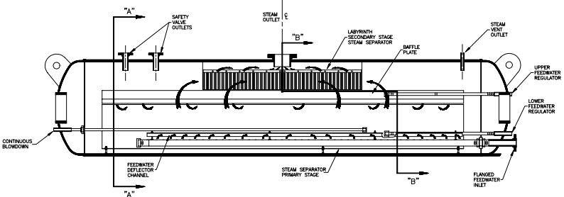
SECTION "C"- SIDE VIEW STEAM DRUM
