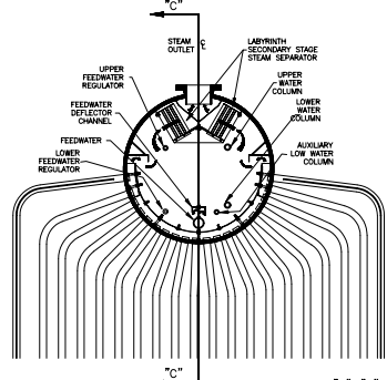
SECTION "B"- END VIEW STEAM DRUM
