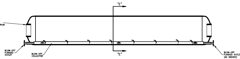
SECTION "D"- SIDE VIEW BOTTOM DRUM
