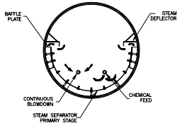
SECTION "A"- FRONT VIEW STEAM DRUM
