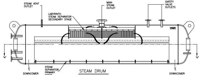
STEAM DRUM
