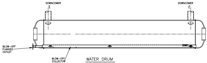
WATER DRUM
