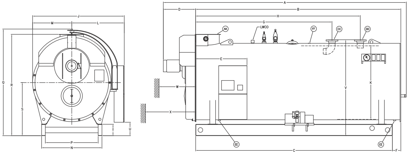
Figure 2. CBEX Elite Hot Water Boiler Dimensions, 100-800 HP
