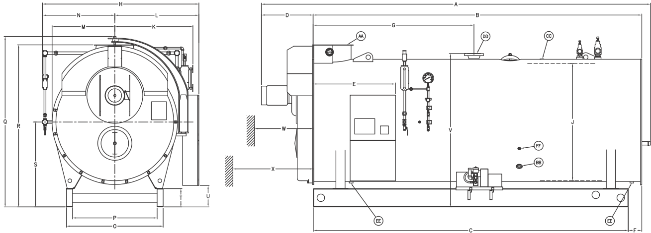
Figure 1. CBEX Elite Steam Boiler Dimensions, 100-800 HP
